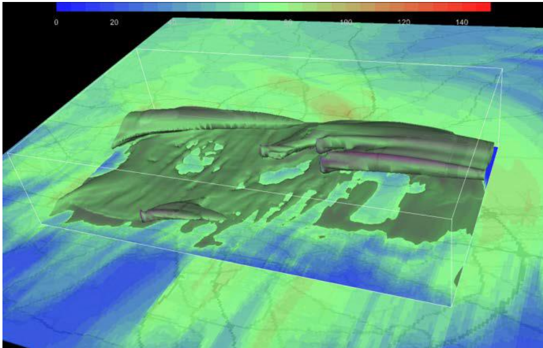
Figure 1. Simulated NO 2 concentration over Munich city for the evening second of February 2015
